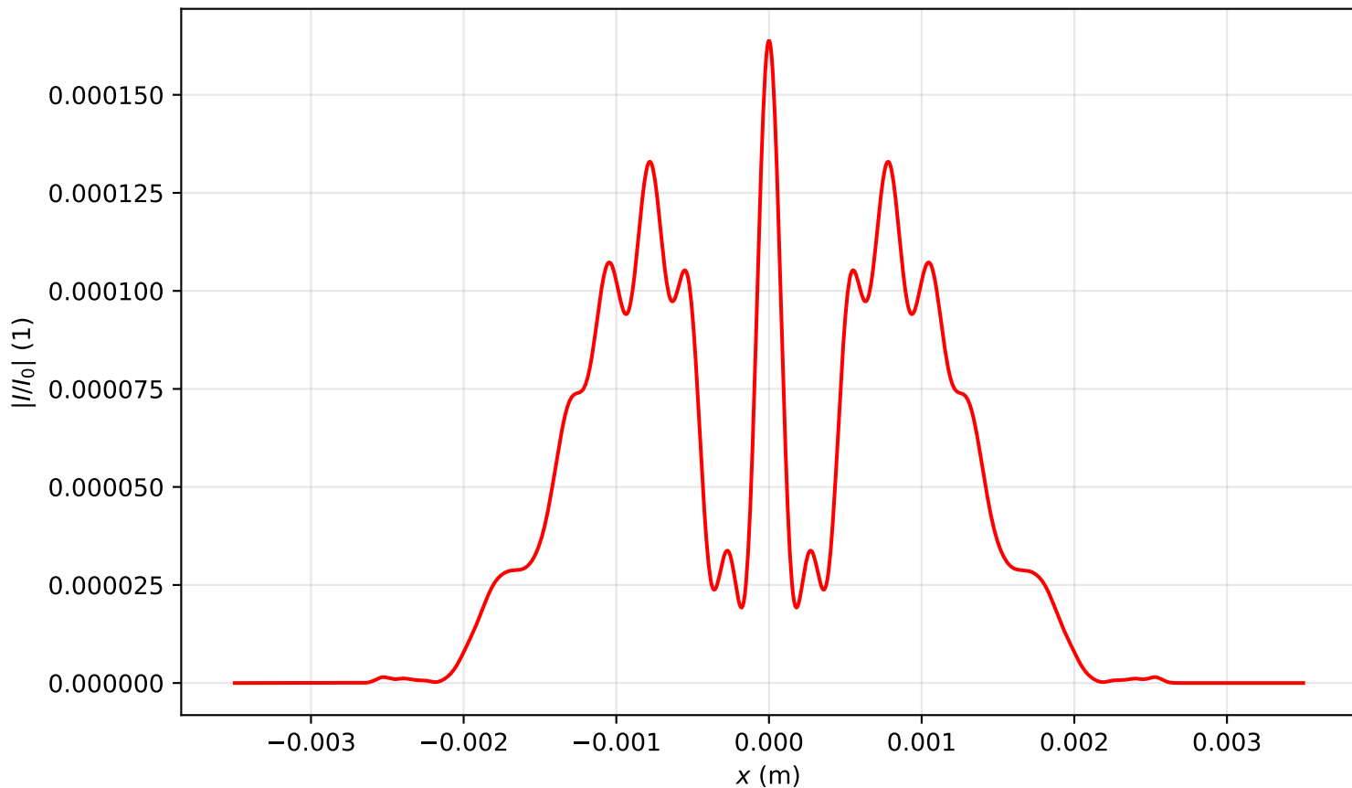
Intensity profile I(x, y = 0, z = 1.353)/I_0 , P_{in}=7.0P_{cr} , artificial time
